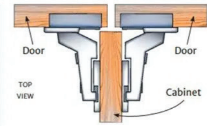
OPTION 2: Half overlay hinge
