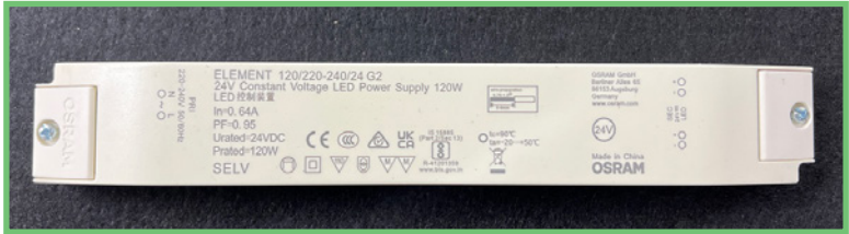
OSRAM TRANSFORMER 120W 24V
