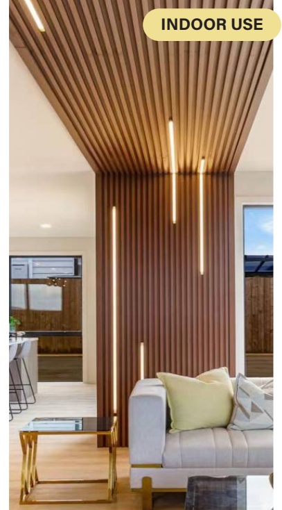
SKU : LED-LP10S or 10B 10 x 10mm Alu. Channel LED Length from 500mm up to 3 Meters (10S)Silver or (10B)Black Colour
